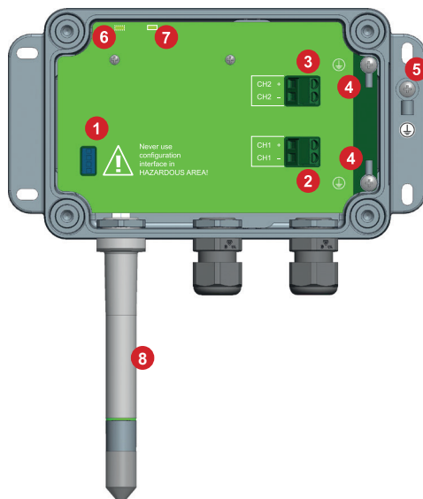
Fig. 8 Electronics board
