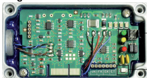
Power LED grün
